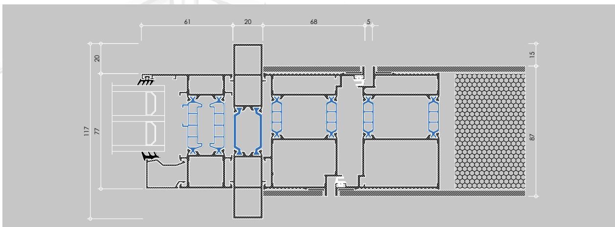
Upper fixed part
